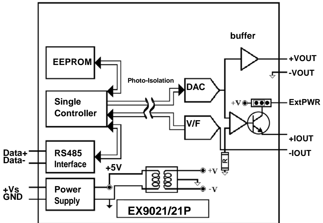
Block Diagram
