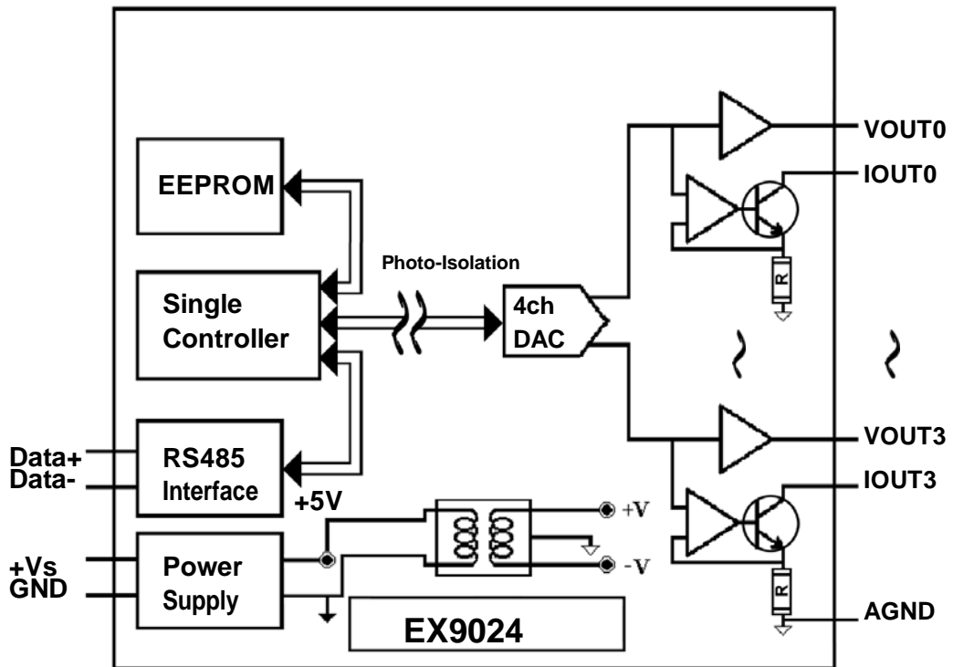
Block Diagram
