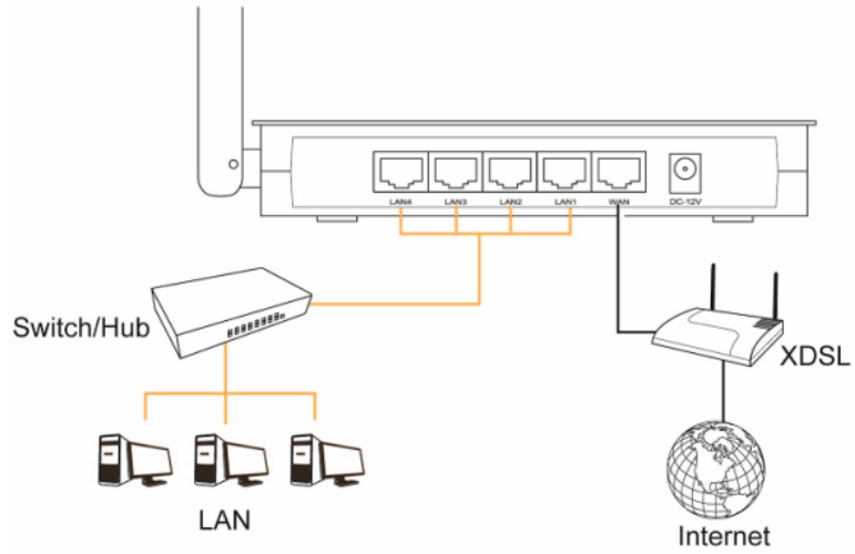
Figure 2-1 Hardware Installation of the EX-92405M2-1
